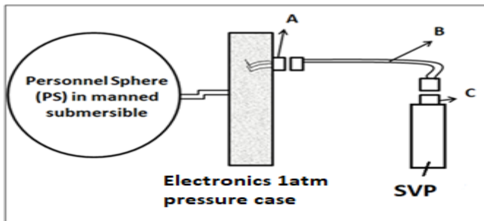
Fig1. Block diagram of SVP interface with Matsya6000
